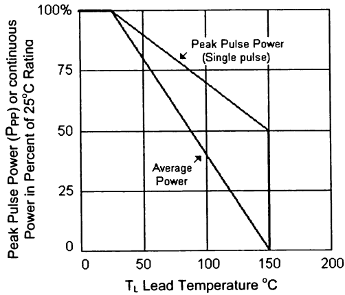
FIGURE 4 Derating Curve
